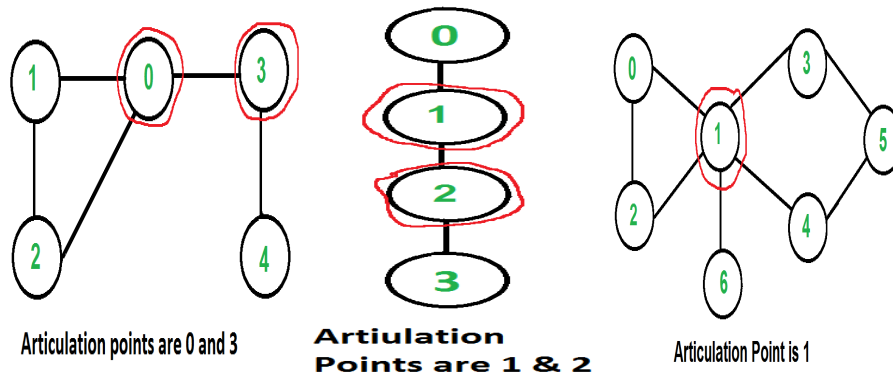
Figure 2.1: Articulation Point
